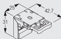
10101 Bracket
