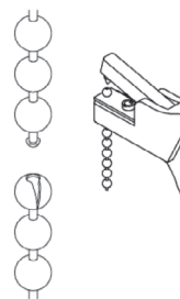
Step 2 - Place bead end into slotted end of 0600 joining plier jaw - apply pressure to pliers and split bead - discard bead and leave complete bead link stalk exposed only - remove chain from plier jaw.
