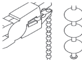
Step 2 - Place bead end into slotted end of 0600 joining plier jaw - apply pressure to pliers and split bead - discard bead and leave complete bead link stalk exposed only - remove chain from plier jaw.
