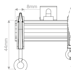
Track end
