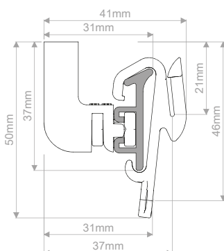
Track installed
