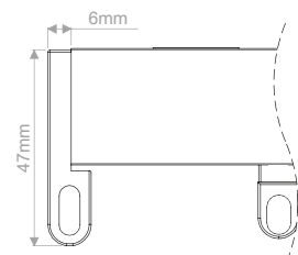
Track end
