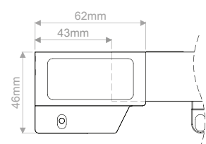
Track end
