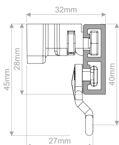
Track installed
