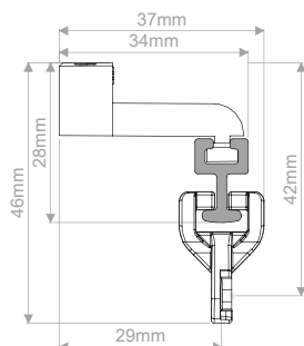
Track installed
