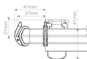
Track end
