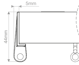
Track end
