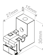
Bracket
