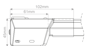
Track end
