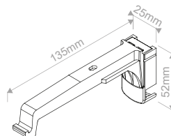
Bracket
