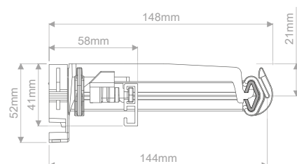
Track installed
