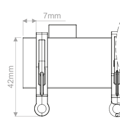
Track end
