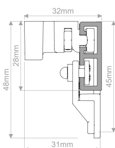
Track installed
