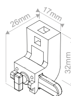
Bracket
