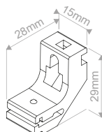
Bracket
