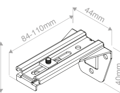
Support Bracket*
