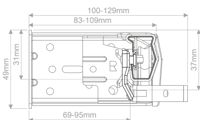
Track installed
