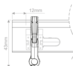
Track end
