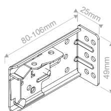
Face Fixing End Bracket
