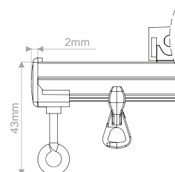
Track end
