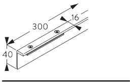
SG 6512 Connection bridge
